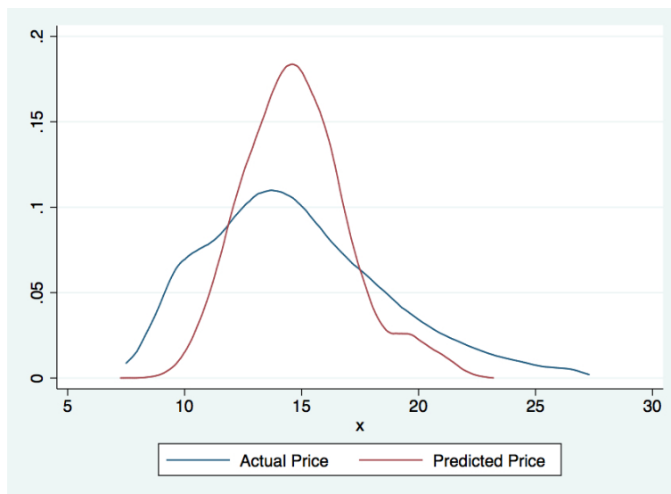
Figure 3: Kernel Densities Comparing Actual and Predicted Prices
